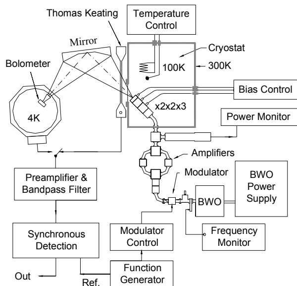
Fig.2. Block diagram of the cryogenic test bench.
