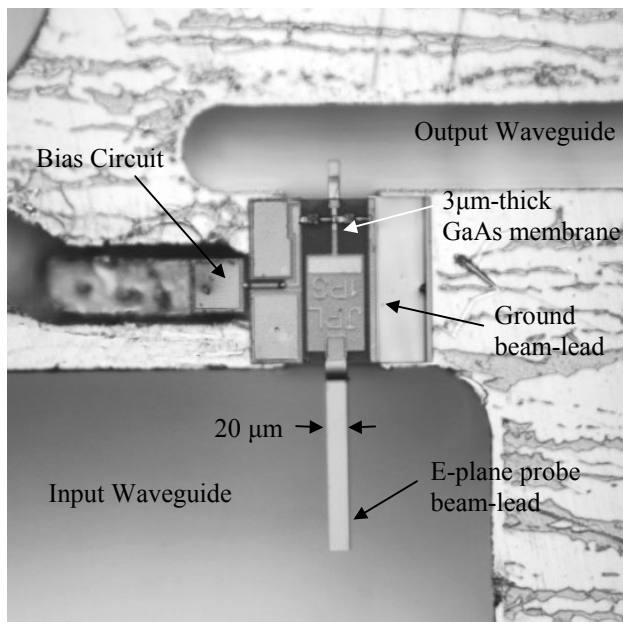
Fig.1. The frameless membrane circuit in the block. The size of the chip without the input and output probes is about 150x160 \mu\text{m} .
