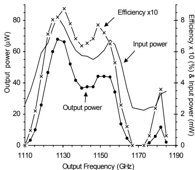
Fig.3. Output power of the 1.2 THz multiplier chain measured at 297K. Bias voltages on the 200 GHz and 400 GHz multipliers are optimized for each frequency.
