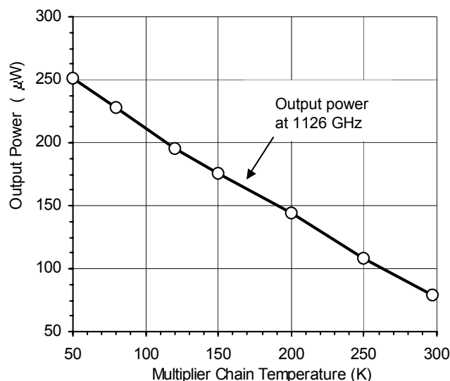
Fig.4. Output power of the 1.2 THz multiplier chain at 1126 GHz measured from 297K to 50K. Bias voltages on the 200 GHz and 400 GHz multipliers are optimized for each temperature (optimized biases are in fact non temperature dependent).
